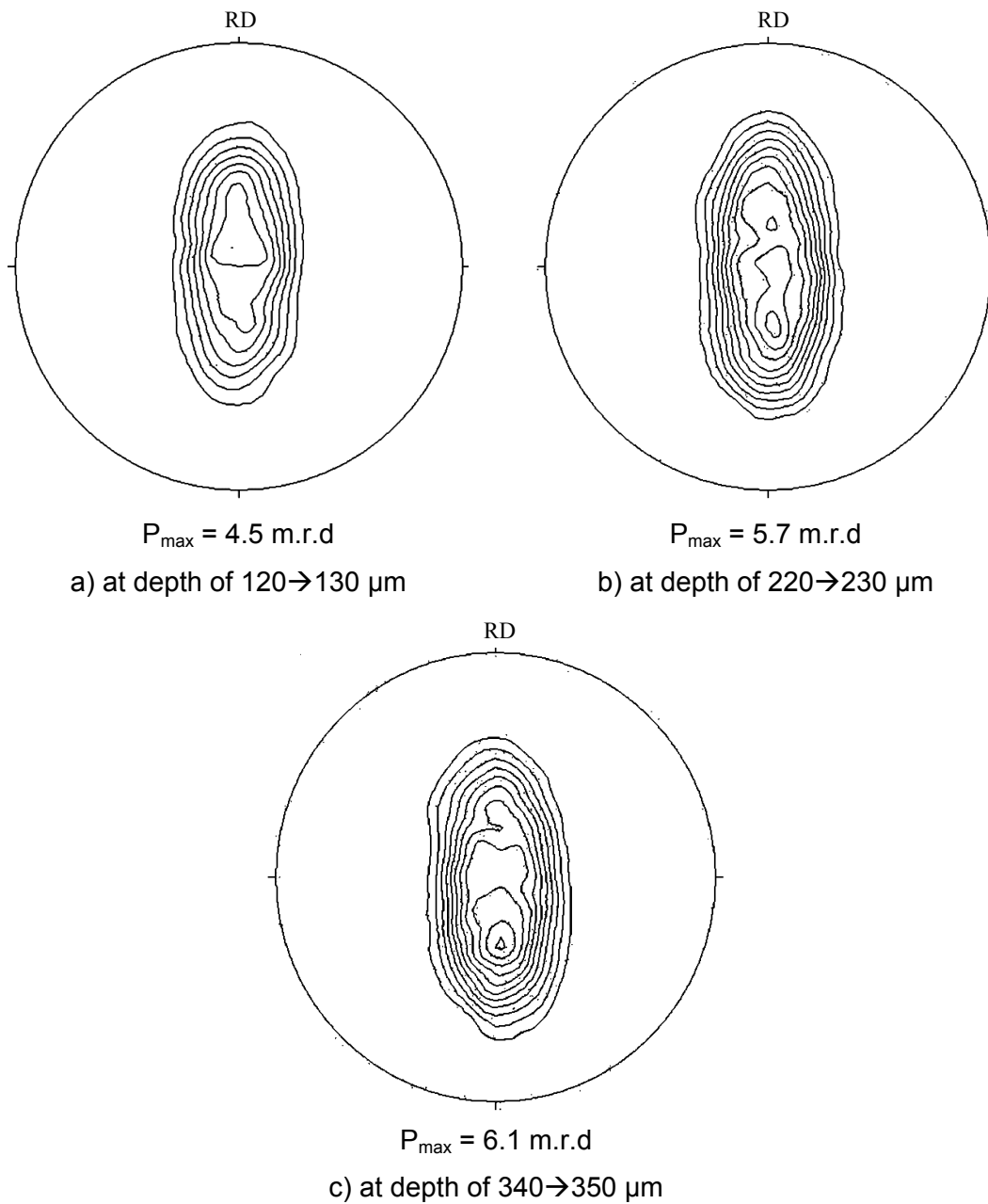
Figure 4.35: Basal pole figures of shot peened Ti-2.5Cu at depth of 120 \rightarrow 130 \mu\text{m} (a), 220 \rightarrow 230 \mu\text{m} (b) and 340 \rightarrow 350 \mu\text{m} (c).
