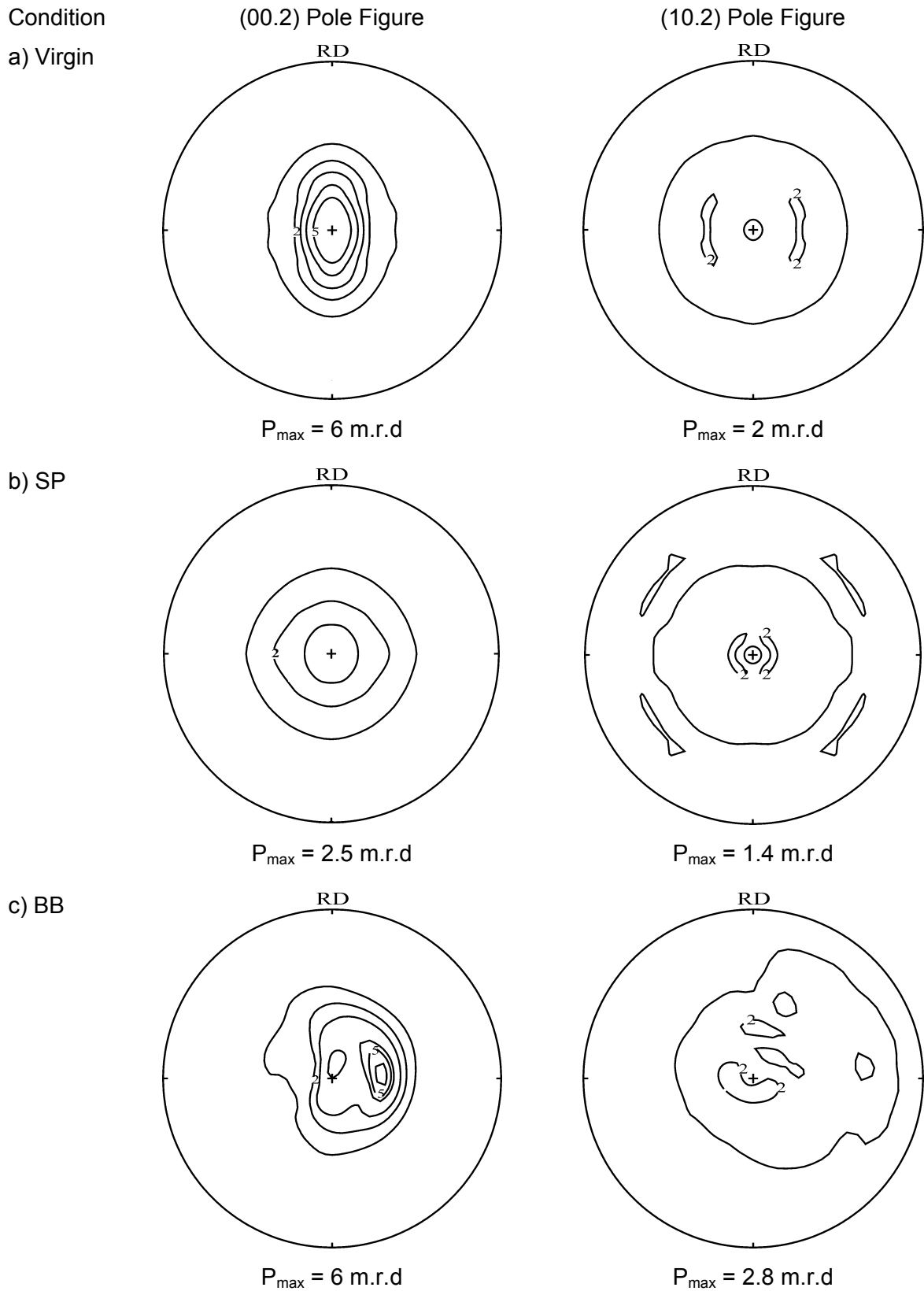
Figure 4.33 (Part I): (00.2) and (10.2) pole figures developed in the surface layer ( 0 \rightarrow 10 \text{ }\mu\text{m} ) of the rolled virgin Ti-2.5Cu (SHT) after SP (b) and BB (c).
