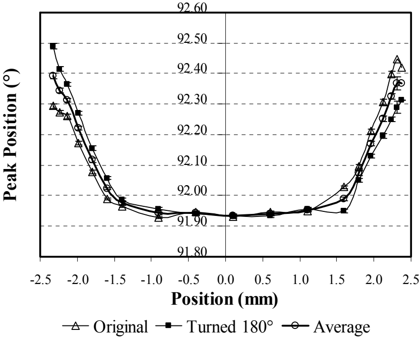
Figure 3.11: Peak position distribution after ball-burnishing (BB).
