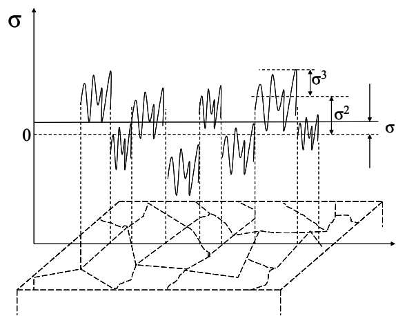
Figure 2.14: Schematic representation of residual stresses of types 1, 2 and 3 [75].
